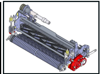
Adjustable bedknife position without dismantling assembly
