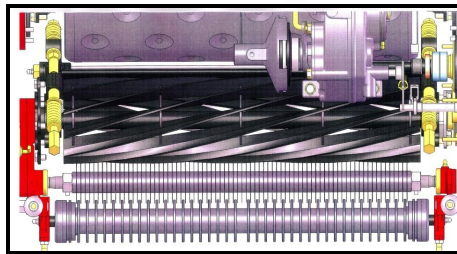
Quick and easy attachment/detachment of attachments for simple maintenance.
